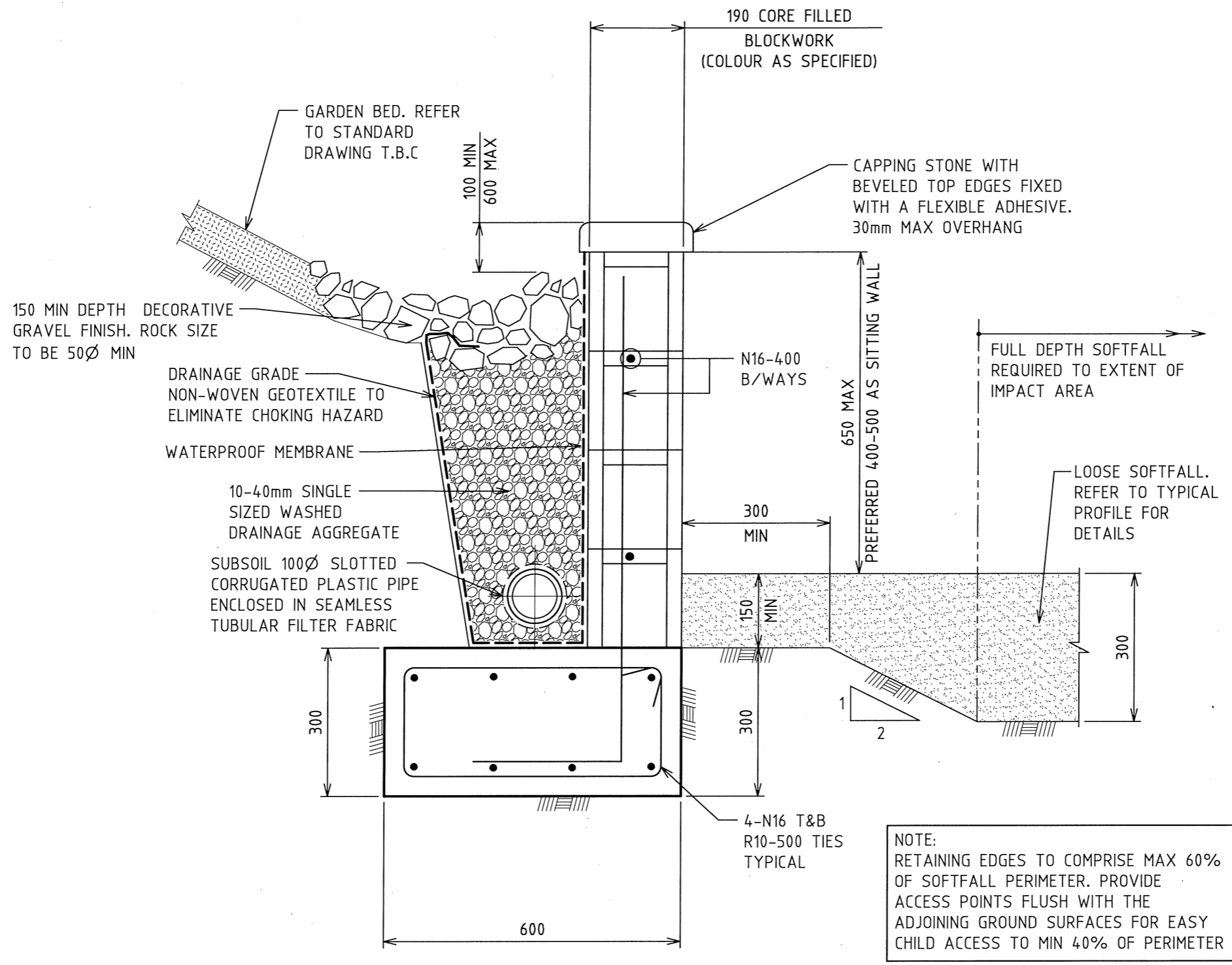
CONCRETE BLOCK RETAINING / SITTING WALL SCALE 1:10
