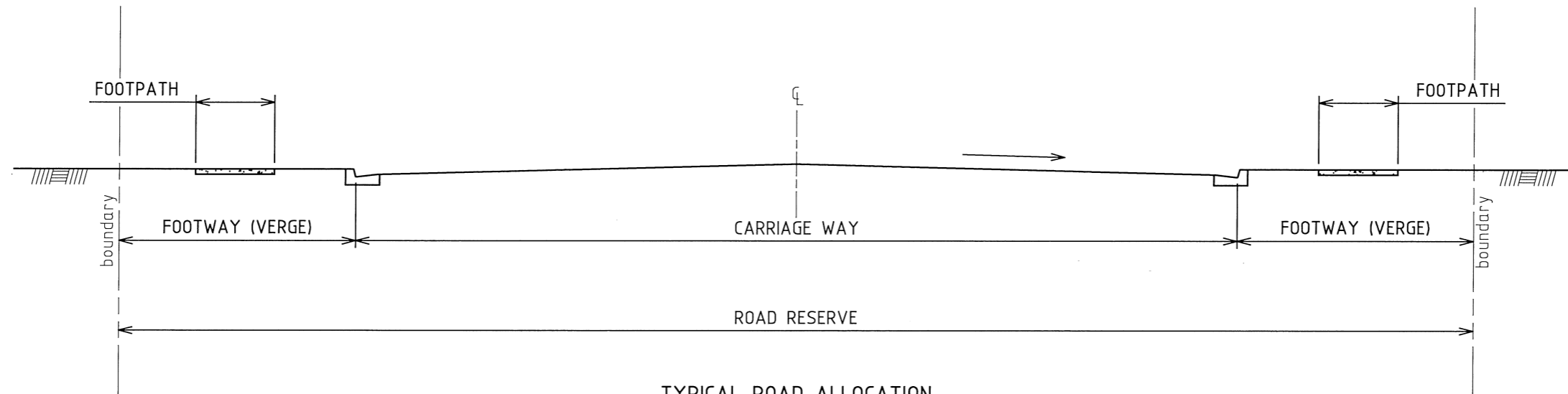
TYPICAL ROAD ALLOCATION SCALE 1:100
